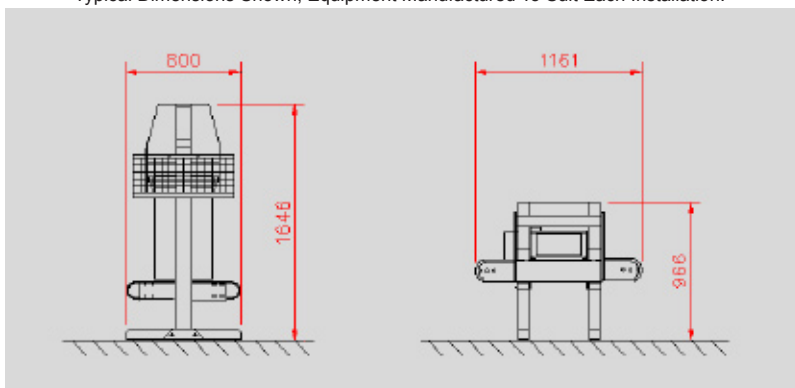
Typical Dimensions Shown, Equipment Manufactured To Suit Each Installation.
